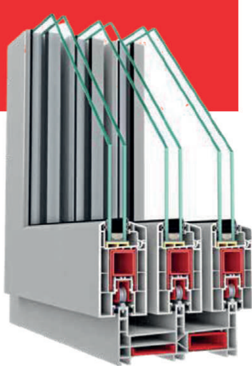
Sliding Three Track double glass
